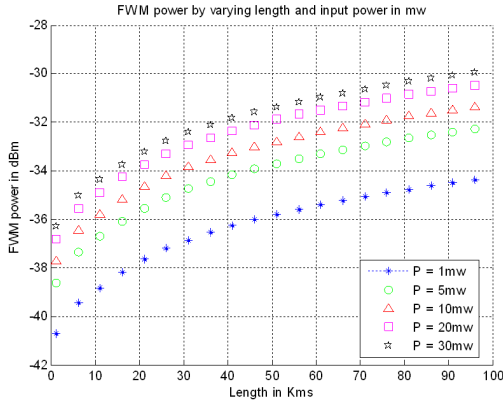
Figure6. FWM Noise Power in dBmVs Length in Kms
