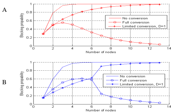
Figure 12. Blocking Probability Vs No Of Nodes For C=25 Using Heuristic Routing Algorithm A. Long Lightpaths B. Shorter Lightpaths.
