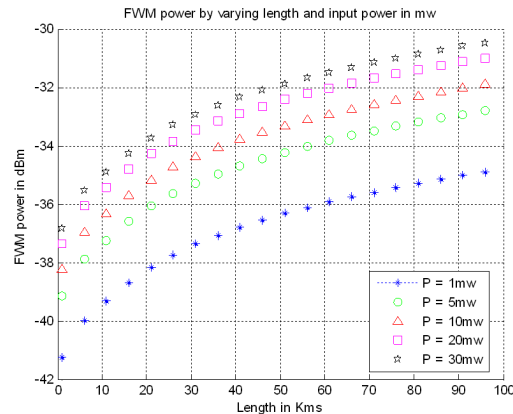
Figure5. FWM Noise Power in dBm Vs Length in Kms
