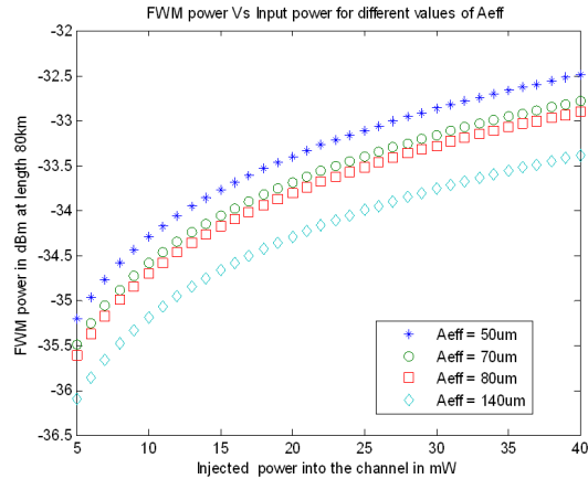
Figure8. FWM Noise Power in dBm Vs Injected power in mW
