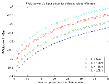
Figure7. FWM Noise Power in dBm Vs Injected power in mW
