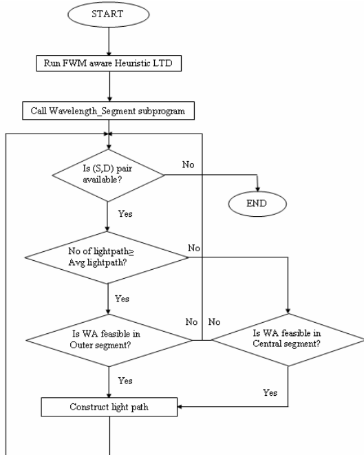
Figure 1. Steps describing Heuristic algorithm and resource allocation
