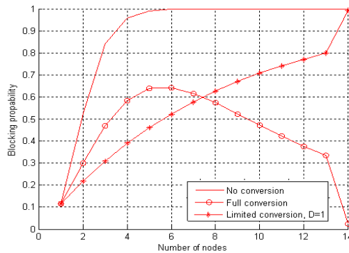
Figure 9. Blocking Probability Vs No of Nodes for C=15 And N=14
