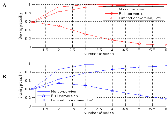
Figure 11. Blocking Probability Vs No Of Nodes For C=15 Using Heuristic Routing Algorithm A. Long Lightpaths B. Shorter Lightpaths.
