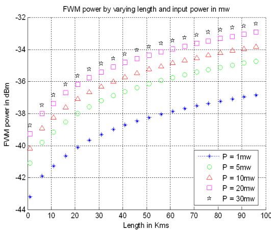
Figure3. FWM Noise Power in dBm Vs Length in Kms
