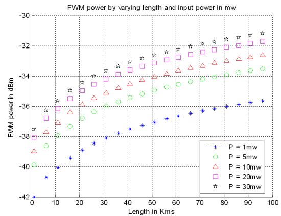
Figure4. FWM Noise Power in dBm Vs Length in Kms
