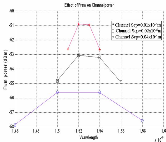
Figure 2. FWM Noise Power Vs Wavelength
