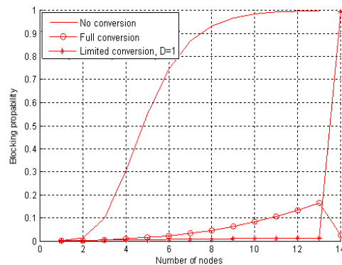
Figure 10. Blocking Probability Vs No of Nodes for C=25 And N=14
